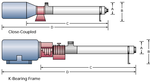
Close-Coupled Pumps
