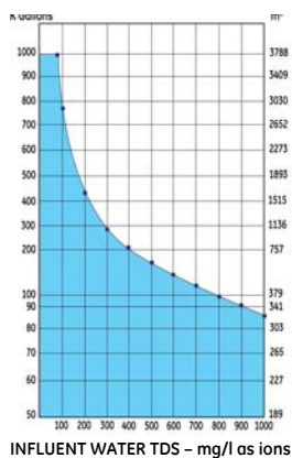
Demineralizer Capacity
