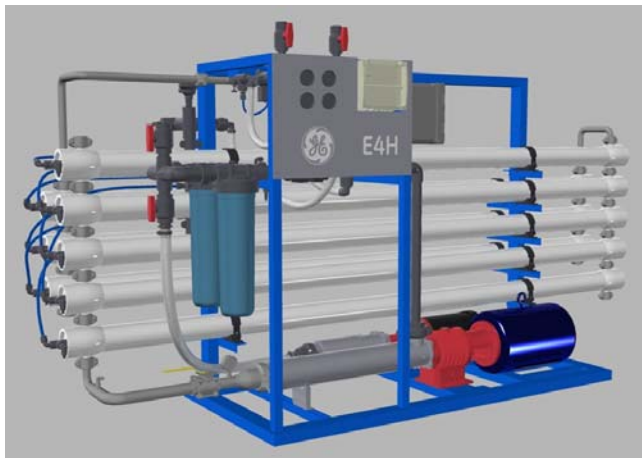
Figure 1: E4H Series 60 Hz
