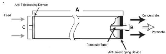
Figure 2: Element Dimensions Diagram - Male (2540)
