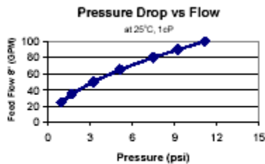
Figure 7: Pressure drop for HWS 8040 elements
