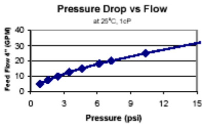
Figure 6: Pressure drop for HWS 4040 elements
