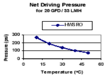
Figure 9: Net Driving Pressure for HWS RO elements
